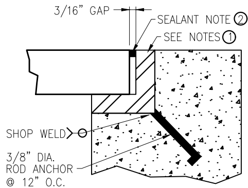
ANCHOR DETAIL
