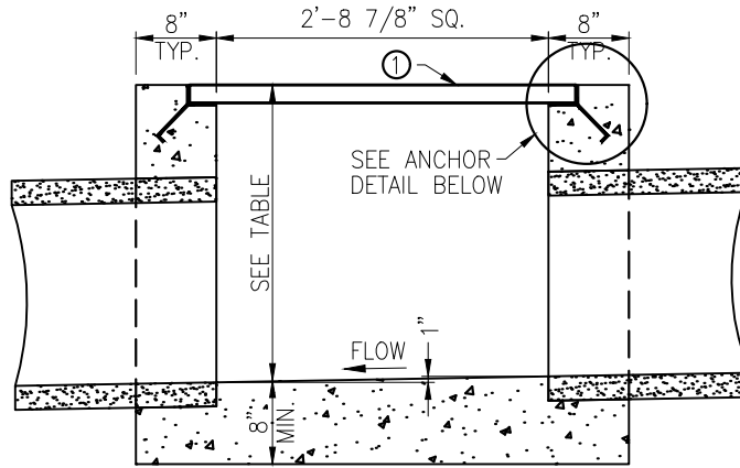
TYPICAL SECTION
